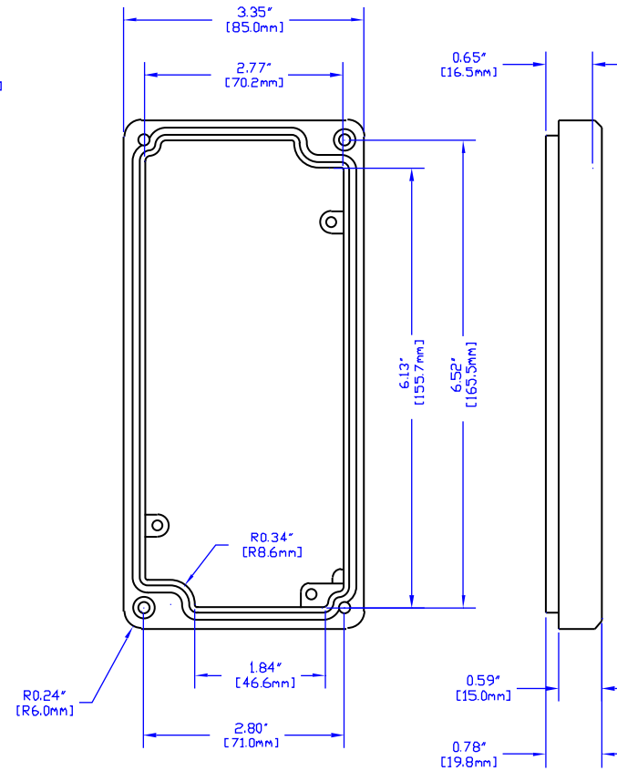
VIEW OF LID (INSIDE)
