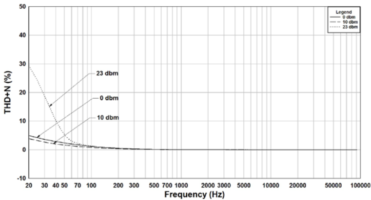
107N Rs=10K, RI=600 THD+N
