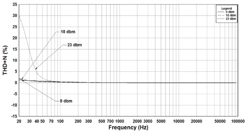
107P Rs=10K, RI=1500 THD+N
