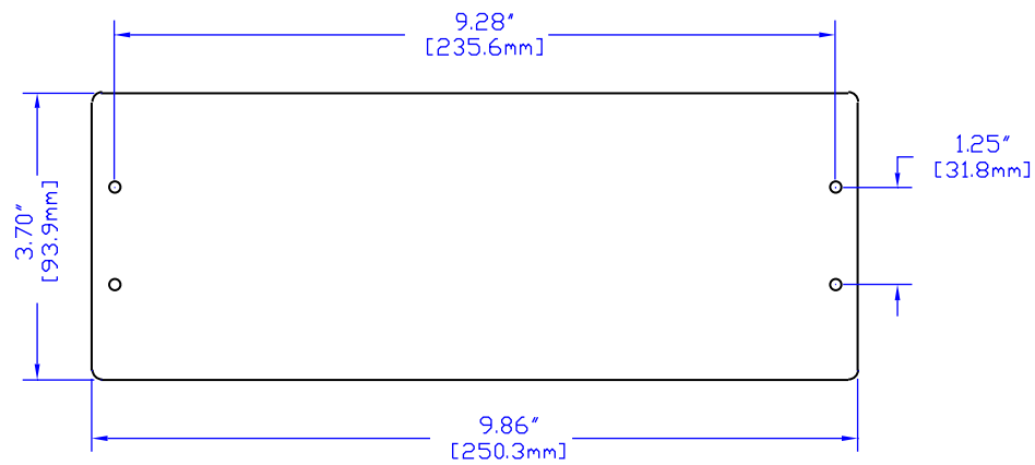
FRONT PANEL
