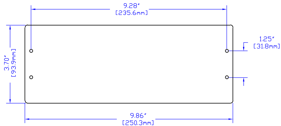
REAR PANEL
