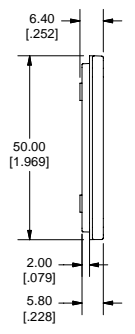
SIDE VIEW OF LID
