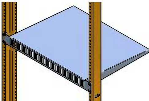
COMPLETE ASSEMBLY
