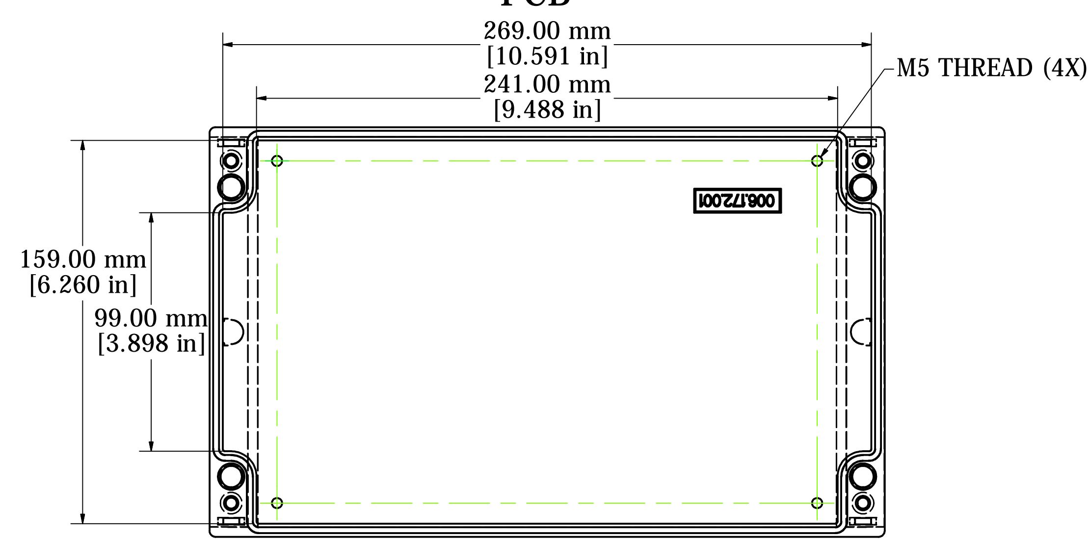
LID - INSIDE VIEW
