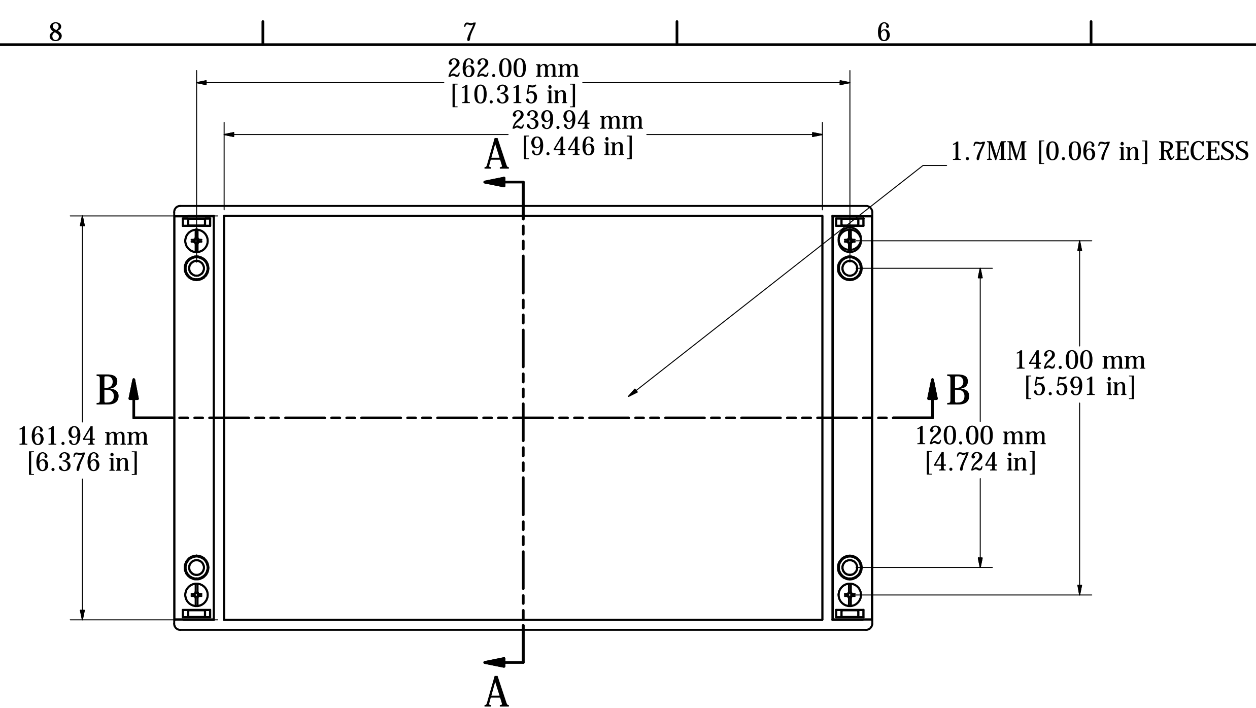
ASSEMBLY - TOP VIEW
