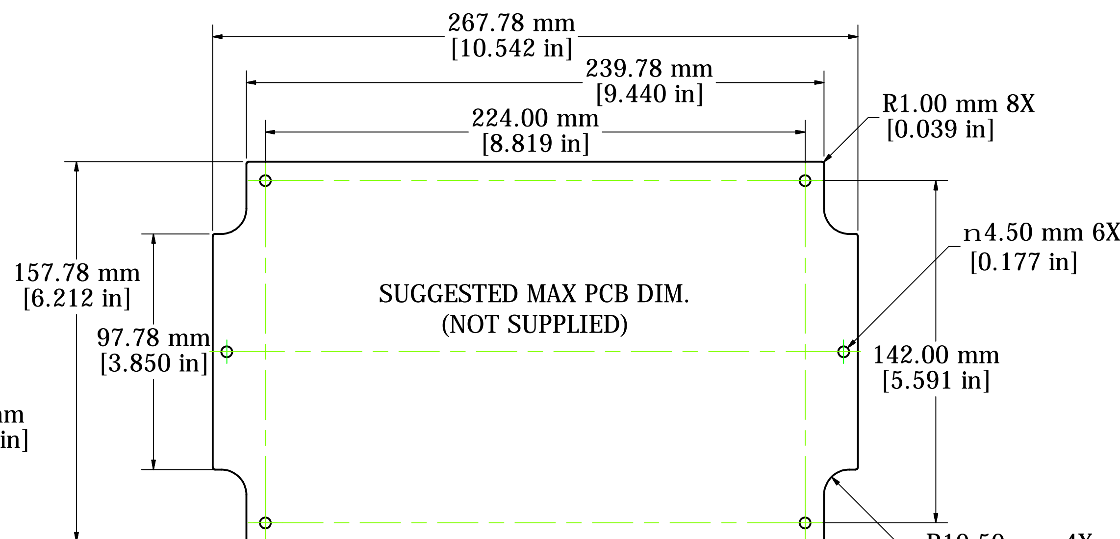
PCB
