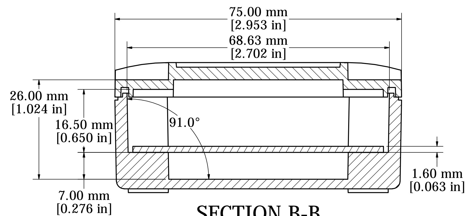
SECTION B-B
