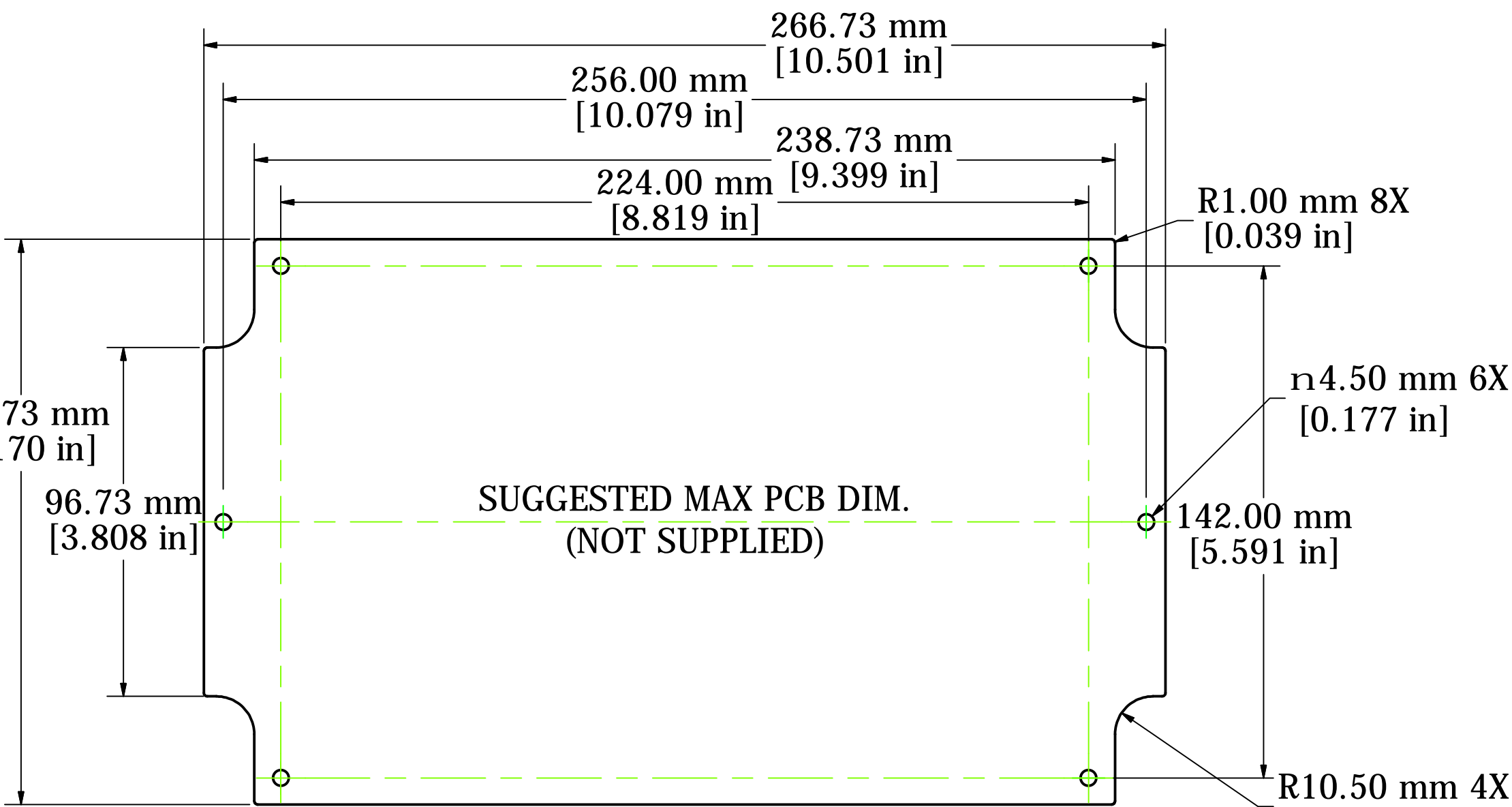
PCB
