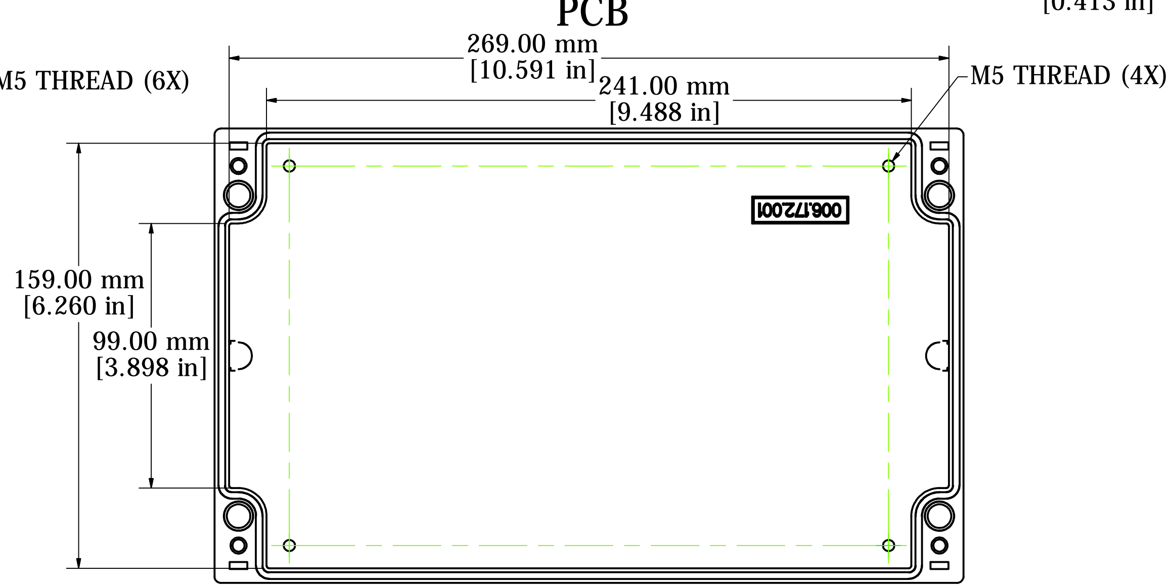
LID - INSIDE VIEW
