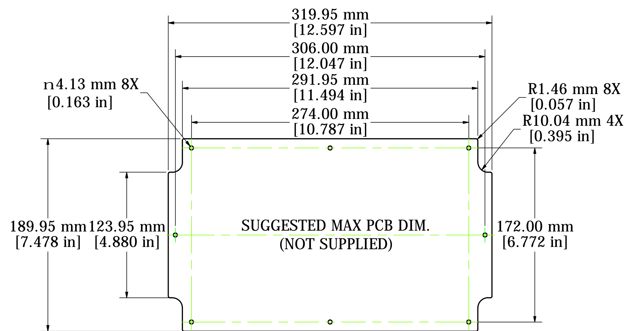
PCB
