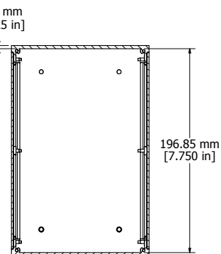
SECTION SS-SS
