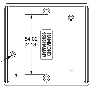
INSIDE BOTTOM
